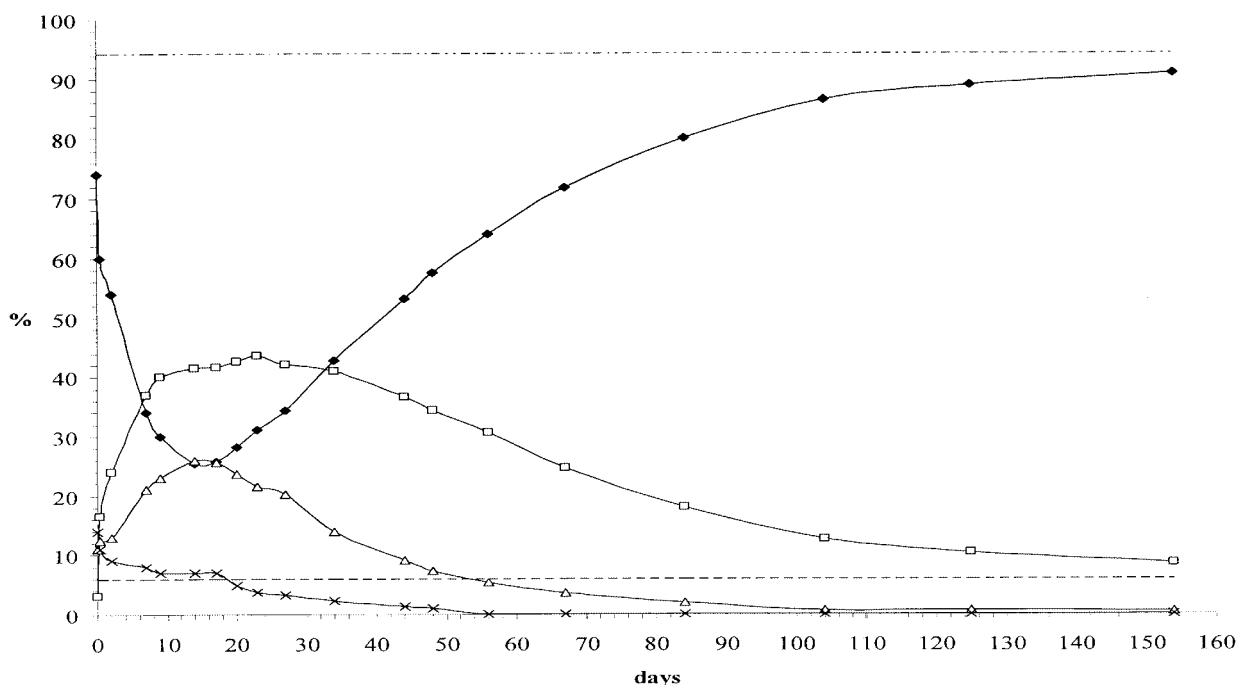
Figure 3. Change of the concentration of ^{13}\text{C} carbonate species as a function of time (black diamonds: ^{13}\text{C}^{16}\text{O}_3^{2-} ; squares: ^{13}\text{C}^{16}\text{O}_2^{18}\text{O}^{2-} ; triangles: ^{13}\text{C}^{16}\text{O}^{18}\text{O}_2^{2-} ; X: ^{13}\text{C}^{18}\text{O}_3^{2-} ; - - - : calculated end-point for ^{13}\text{C}^{16}\text{O}_3^{2-} ; - - - : calculated end-point for ^{13}\text{C}^{16}\text{O}_2^{18}\text{O}^{2-}
